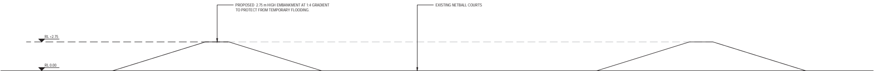
1 TYPICAL ELEVATION - NETBALL COURTS SCALE 1 : 500
