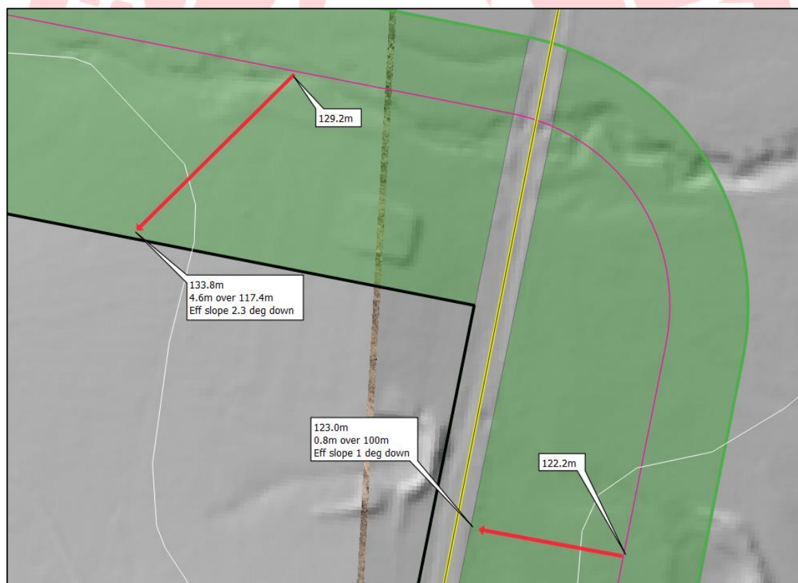
Figure 4 LiDAR 1m DEMS slope analysis
